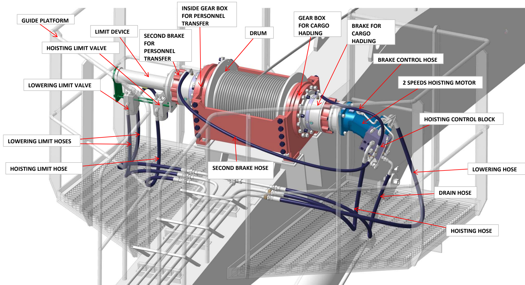
MODIFIED 10TON PERSONNEL TRANSFER HOISTING WINCH
